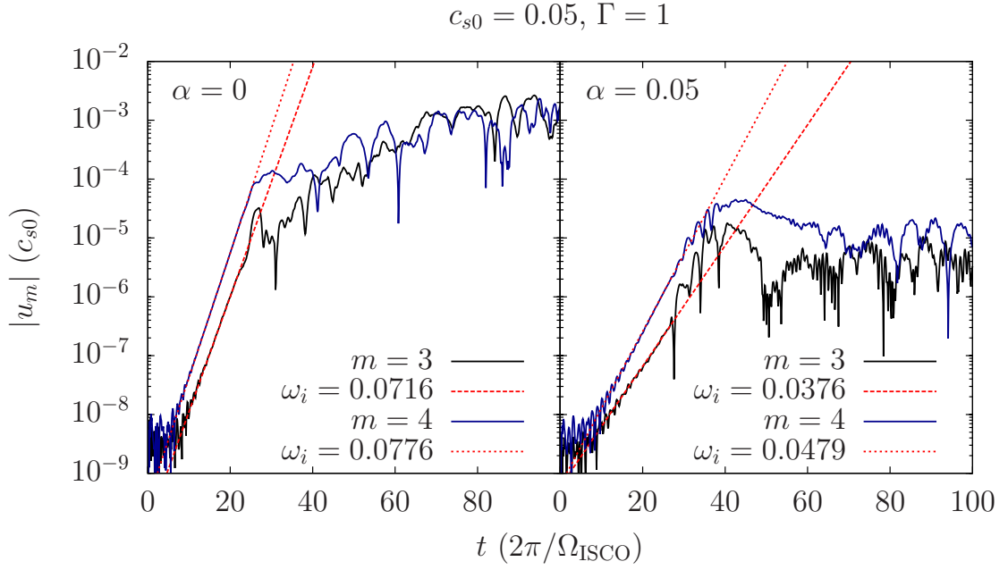
Figure 2.7: Evolution of the m = 3 and m = 4 components of radial velocity [|u_m|, \text{ in units of } c_{s0} = c_s(r_{\text{ISCO}})] at r = 1.05 for a typical run, showing exponential growth of trapped p -mode amplitudes, for zero and non-zero \alpha . The dashed and dotted lines show the exponential curves used to fit the mode growth rates. The reduction in growth rate and reduced saturation amplitude due to viscosity can be seen.
