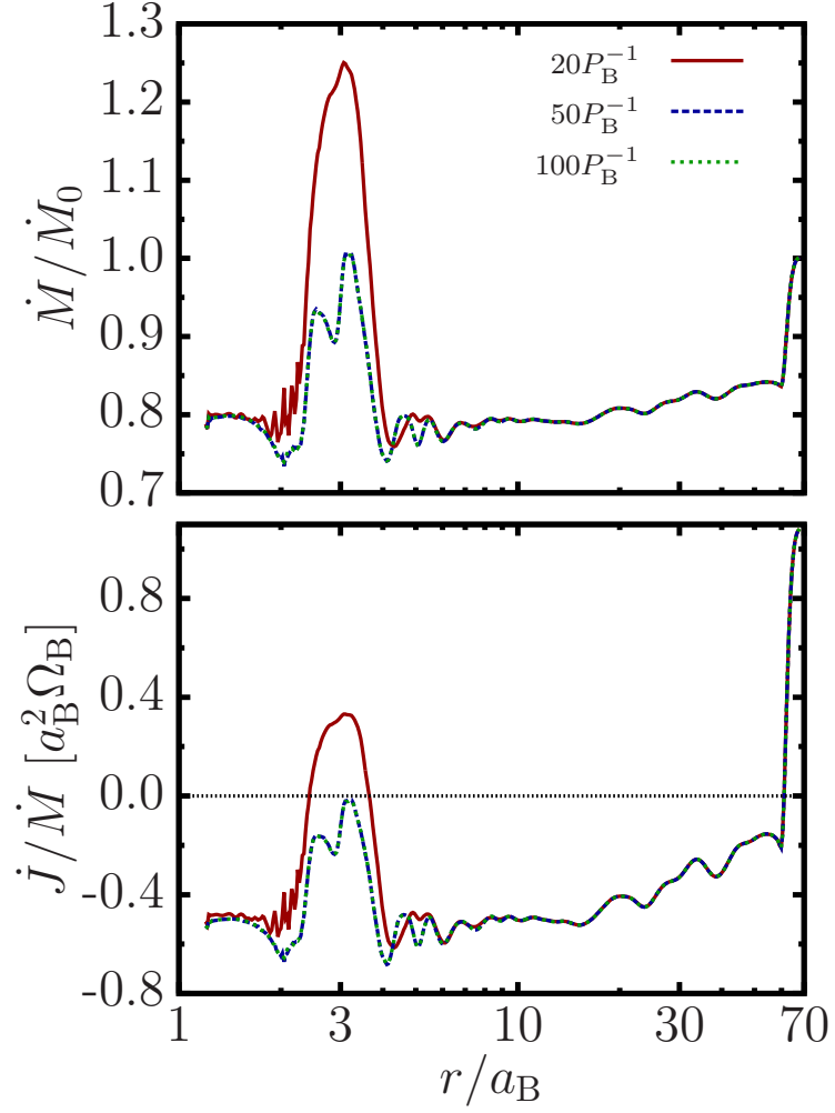
Figure 6.15: Time averaged \dot{M} and \dot{J} for the simulation with q_B = 1.0, e_B = 0.2, \alpha = 0.05 , each taken over 50 binary orbits, with several time sampling rates, as indicated. Flatter profiles are obtained by using higher time sampling rates.
